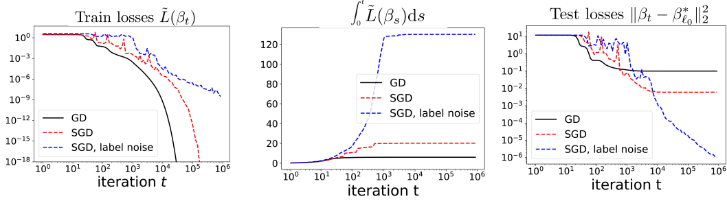
Figure 5: Sparse regression (see Section 5.1 for the detailed experimental setting), illustration of the benefits of using label noise. All experiments are initialised at \alpha = 0.01 . Left : The use of label noise slows down the convergence of the effective training loss \tilde{L} . Middle and right : the value of the integral of the slowed down loss \tilde{L} is much higher for the recursion with label noise, leading to a solution which generalises much better.
